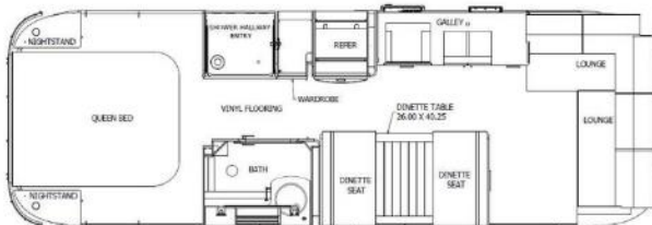
28RB POTTERY BARN - QUEEN FLOOR PLAN
