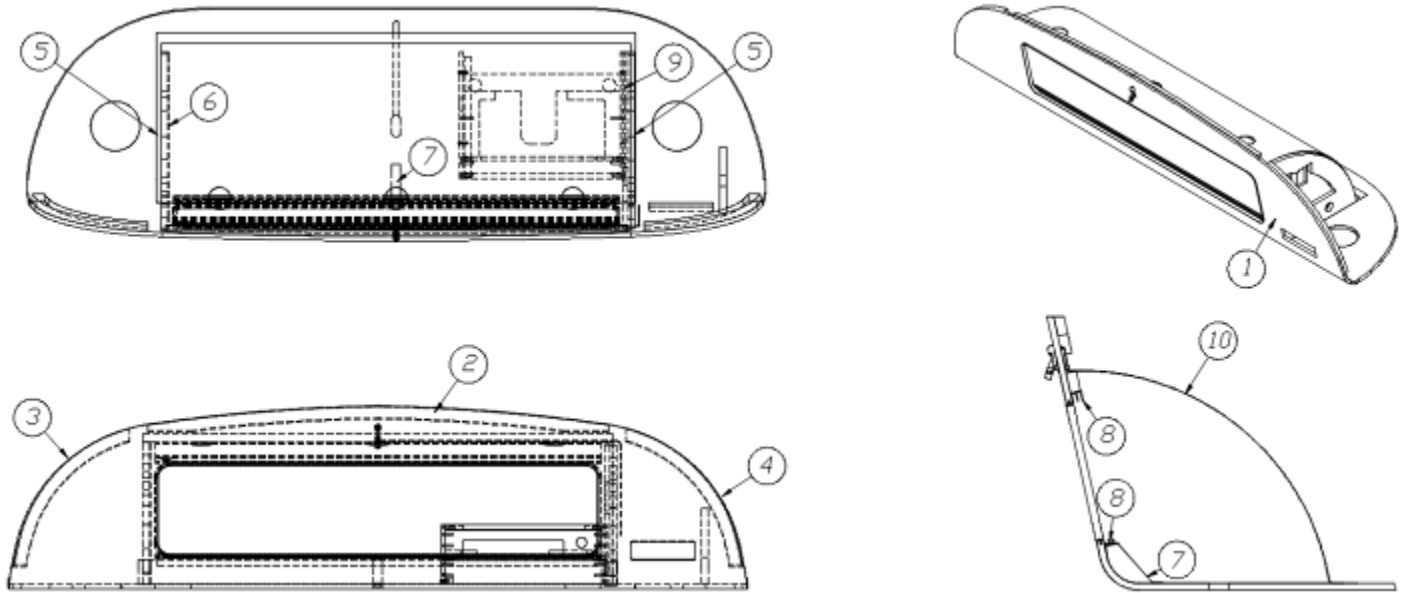
969142 Front Liner Roof locker
