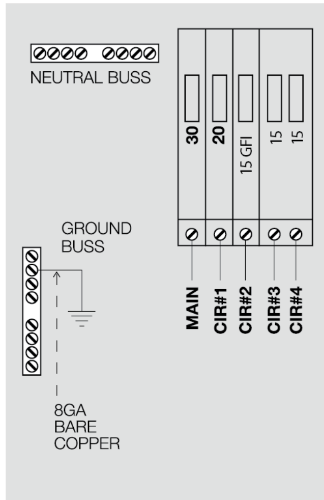
Inset "A" Breaker Layout
