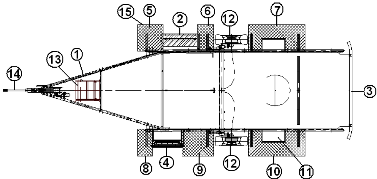
Chassis Diagram, 534
